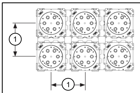
1 Centre distance
