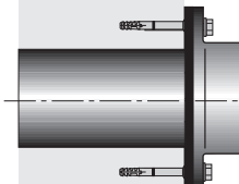
HSI 90-DF Flange for do- weling in front of core drillings Ø max. = 90 mm
