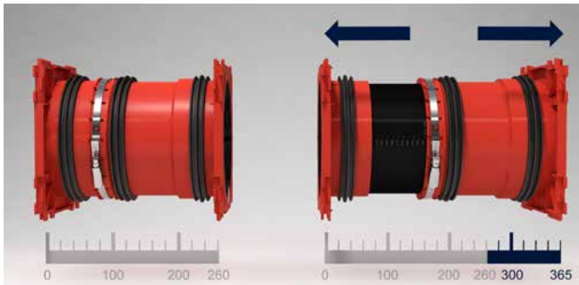
continuously adjustable to the required wall thickness, example HSI150 1x1 K2 Varia 260-365
