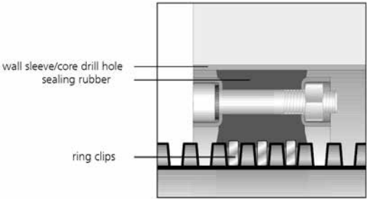
Detailed view: Clip ring/seal
