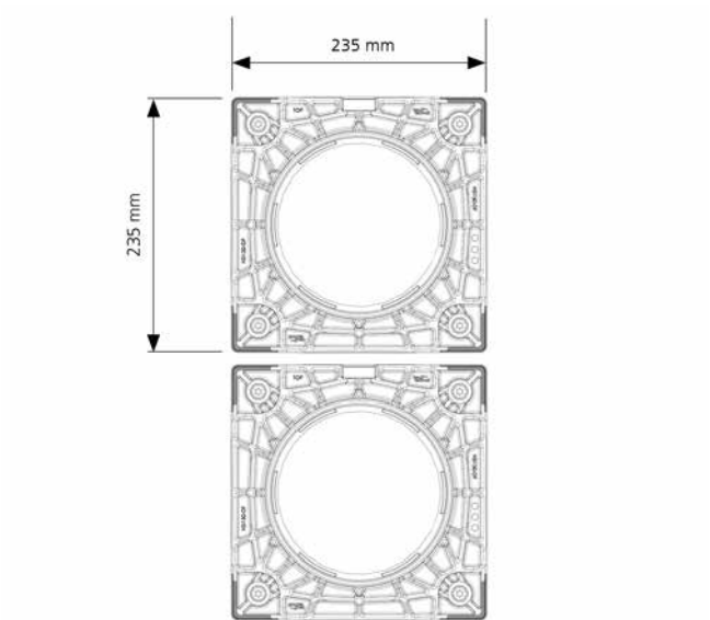
Multiple arrangement HSI150 DFK
