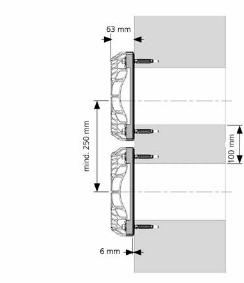
spacing dimensions
