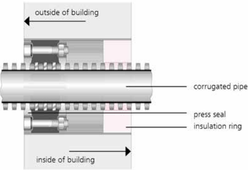
Sectional drawing: Positioning in the bore
